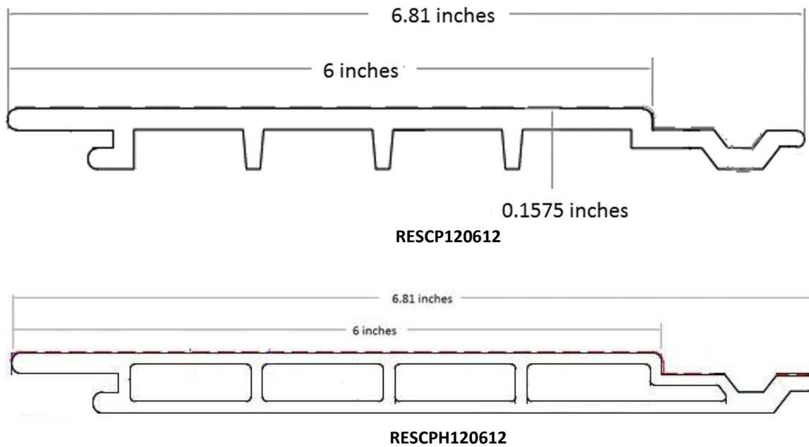
FIGURE 1 – RESYSTA 6" SIDING
