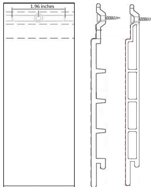
FIGURE 2 – INSTALLATION
