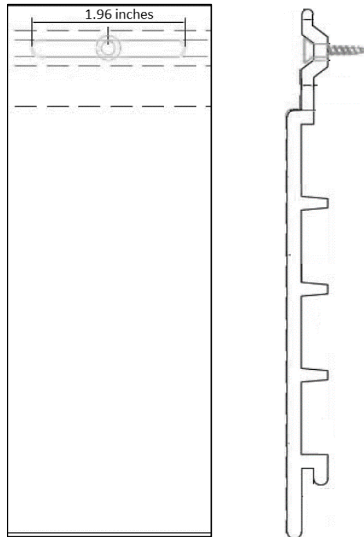
Figure 2 – Installation
