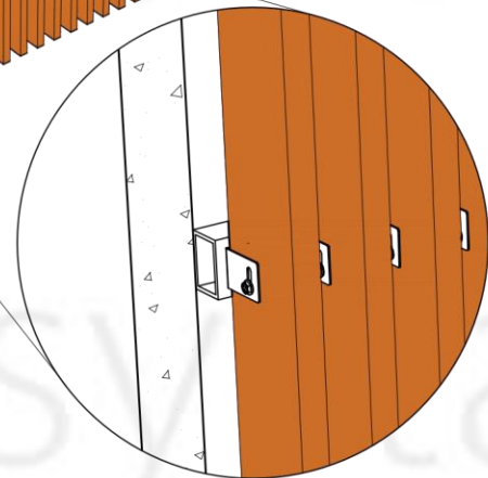
DETAIL-2.0
