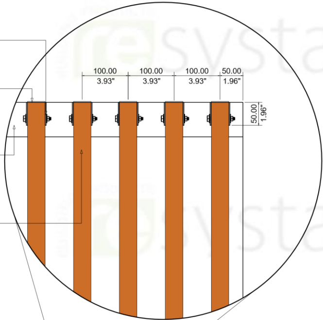
DETAIL - 4.0
