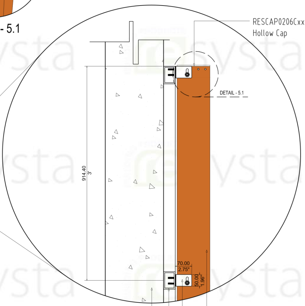
SECTION
