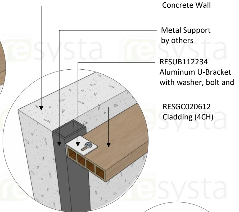
ISOMETRIC Detail
