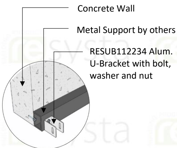
SECTION DETAIL 3 Lower End U-Bracket
