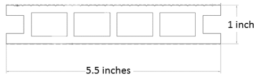
Figure 2 – Platinum Decking
