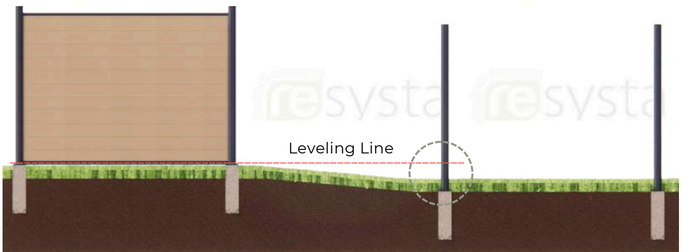
ELEVATION Fence System
