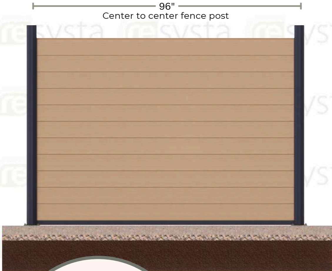
ELEVATION Fence System
