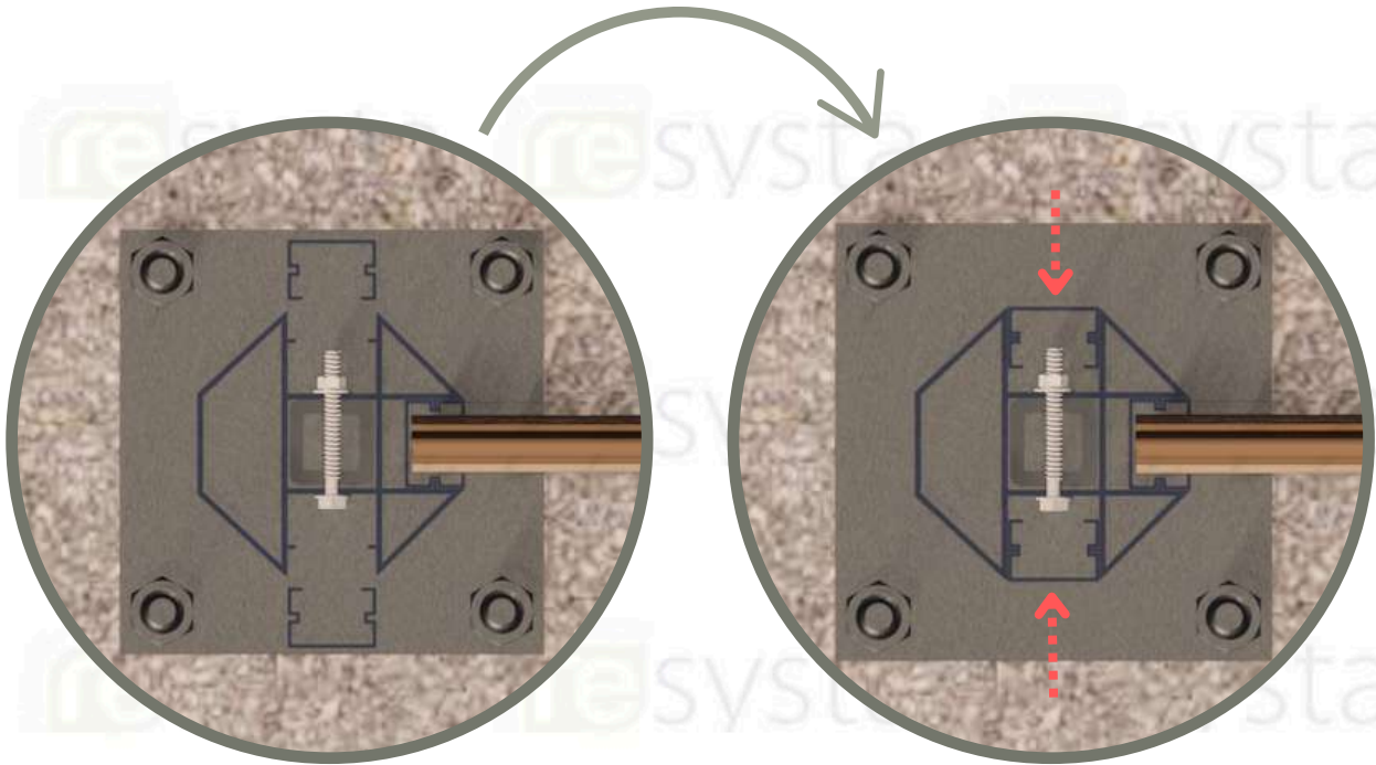
TOP VIEW - SECTION A Fence System
