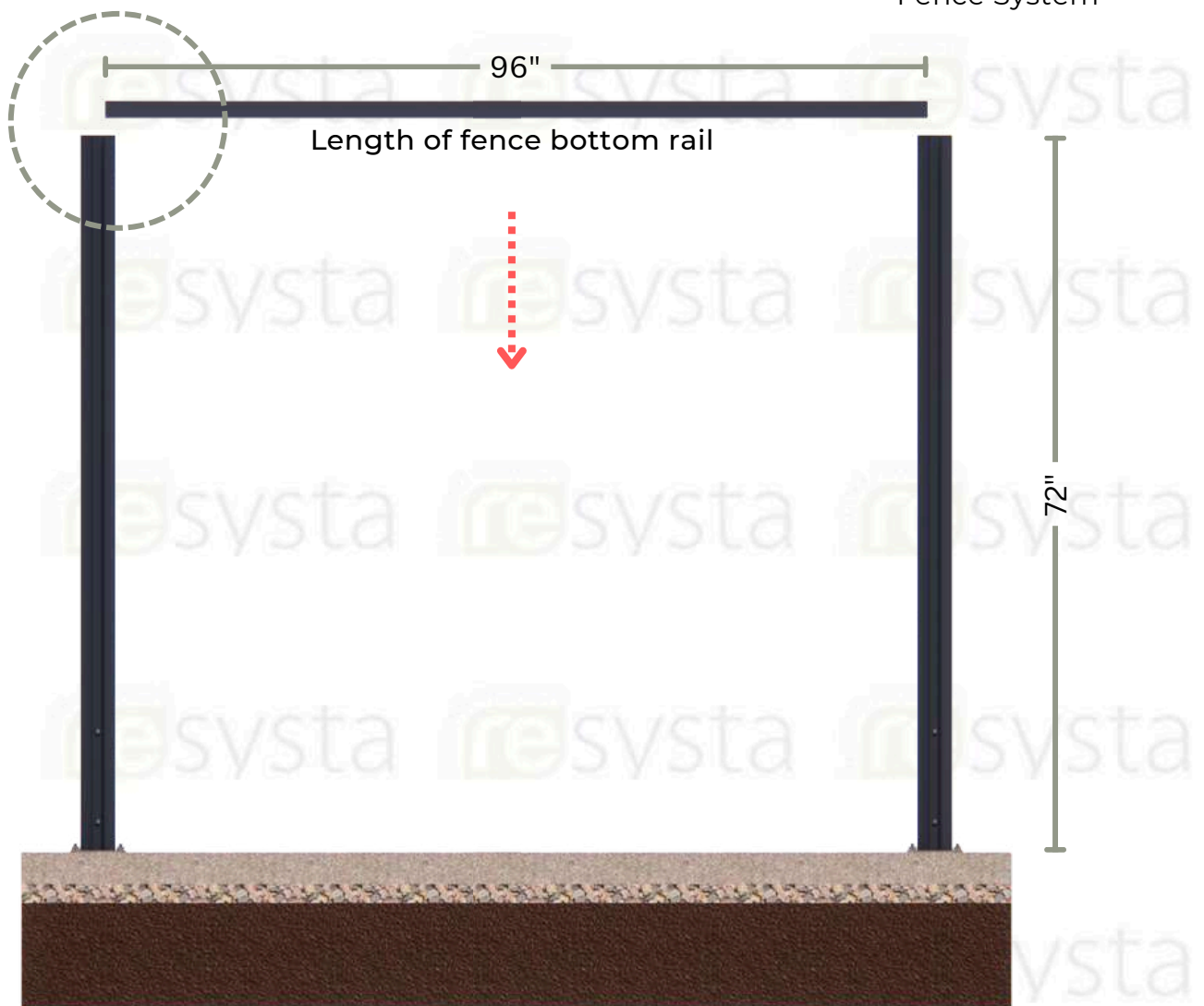
ELEVATION Fence System
