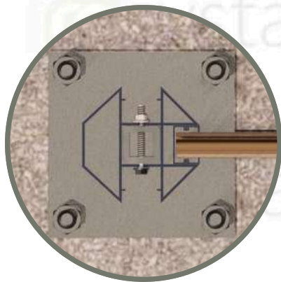
TOP VIEW DETAIL
