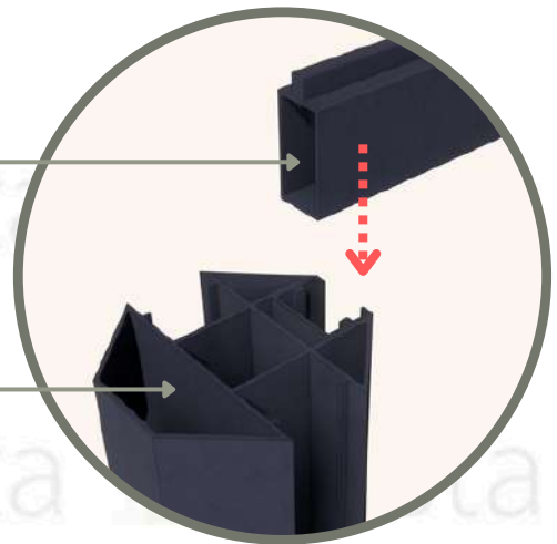
ISOMETRIC DETAIL Fence System
