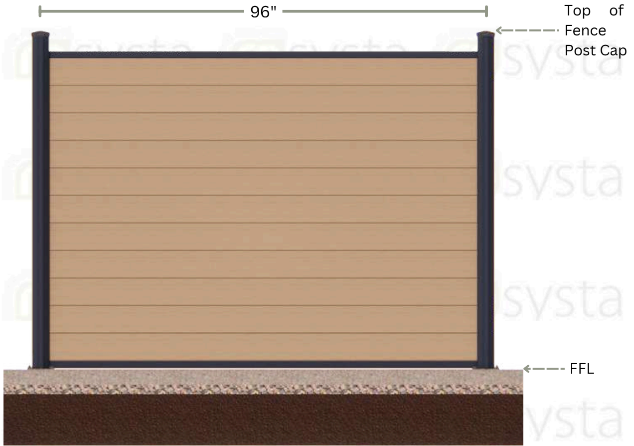
ELEVATION Fence System
