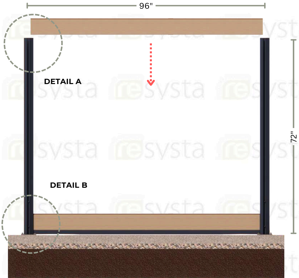
ELEVATION Fence System
