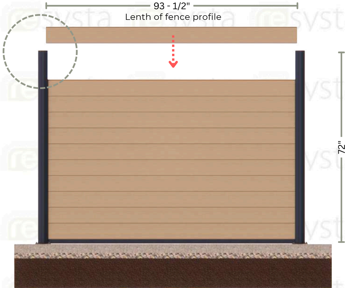
ELEVATION Fence System
