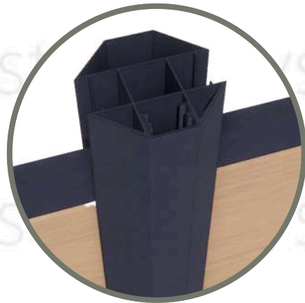
ISOMETRIC VIEW Linear Detail
