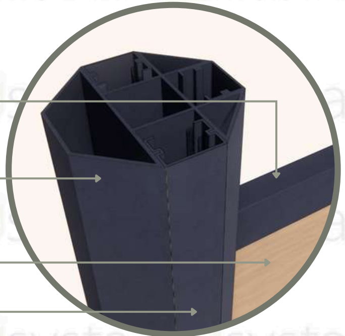
ISOMETRIC DETAIL Fence System
